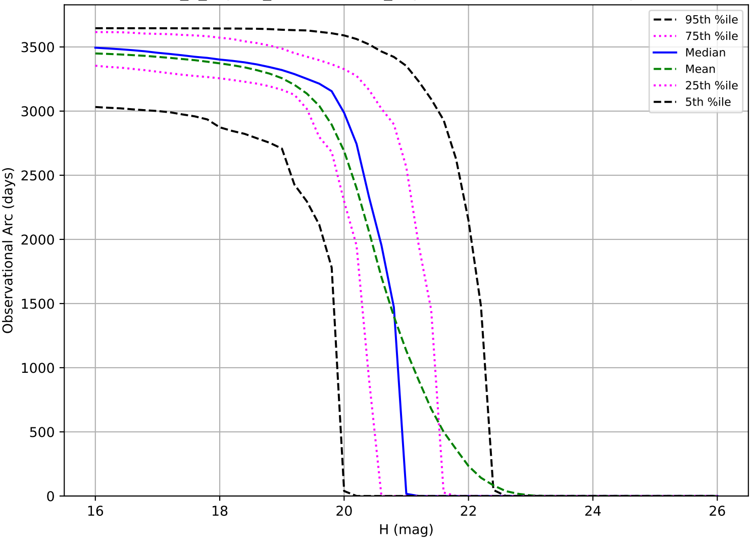
internal_u_expt45_nscale0.9v3.4_10yrs: Observational Arc Length MBA
