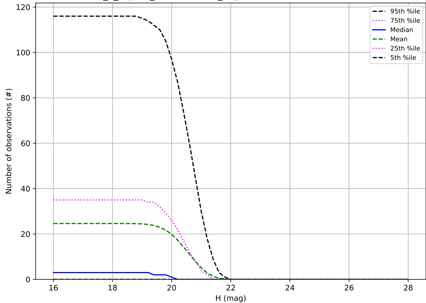
internal_u_expt45_nscale0.9v3.4_10yrs: Number of observations Vatira
