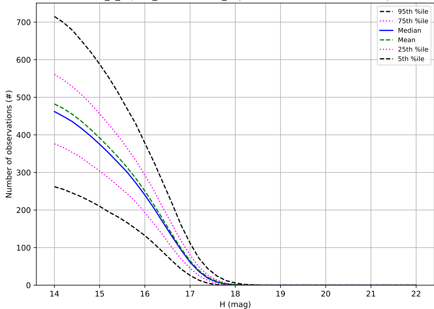
internal_u_expt45_nscale0.9v3.4_10yrs: Number of observations Trojan
