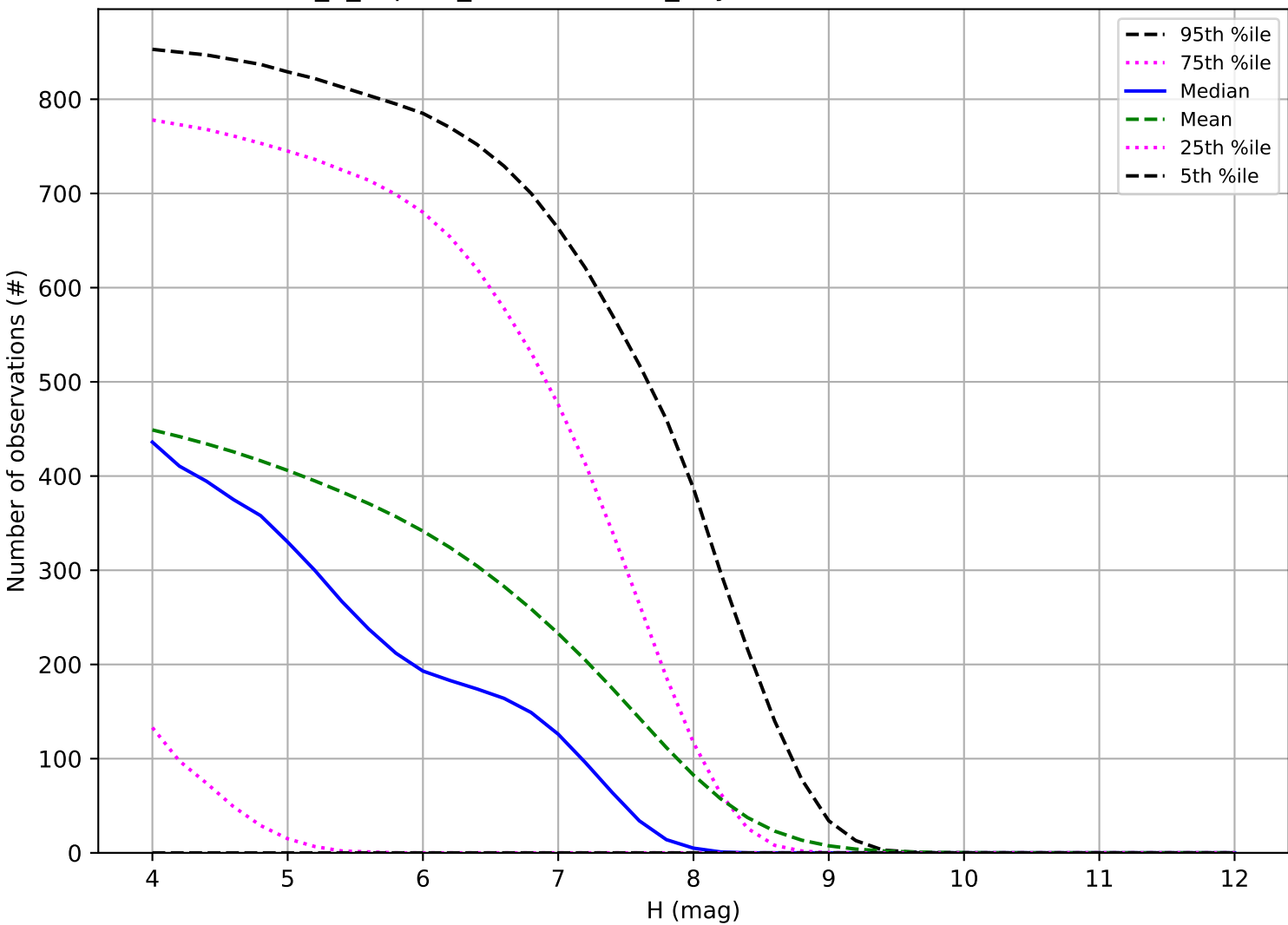
internal_u_expt45_nscale0.9v3.4_10yrs: Number of observations TNO
