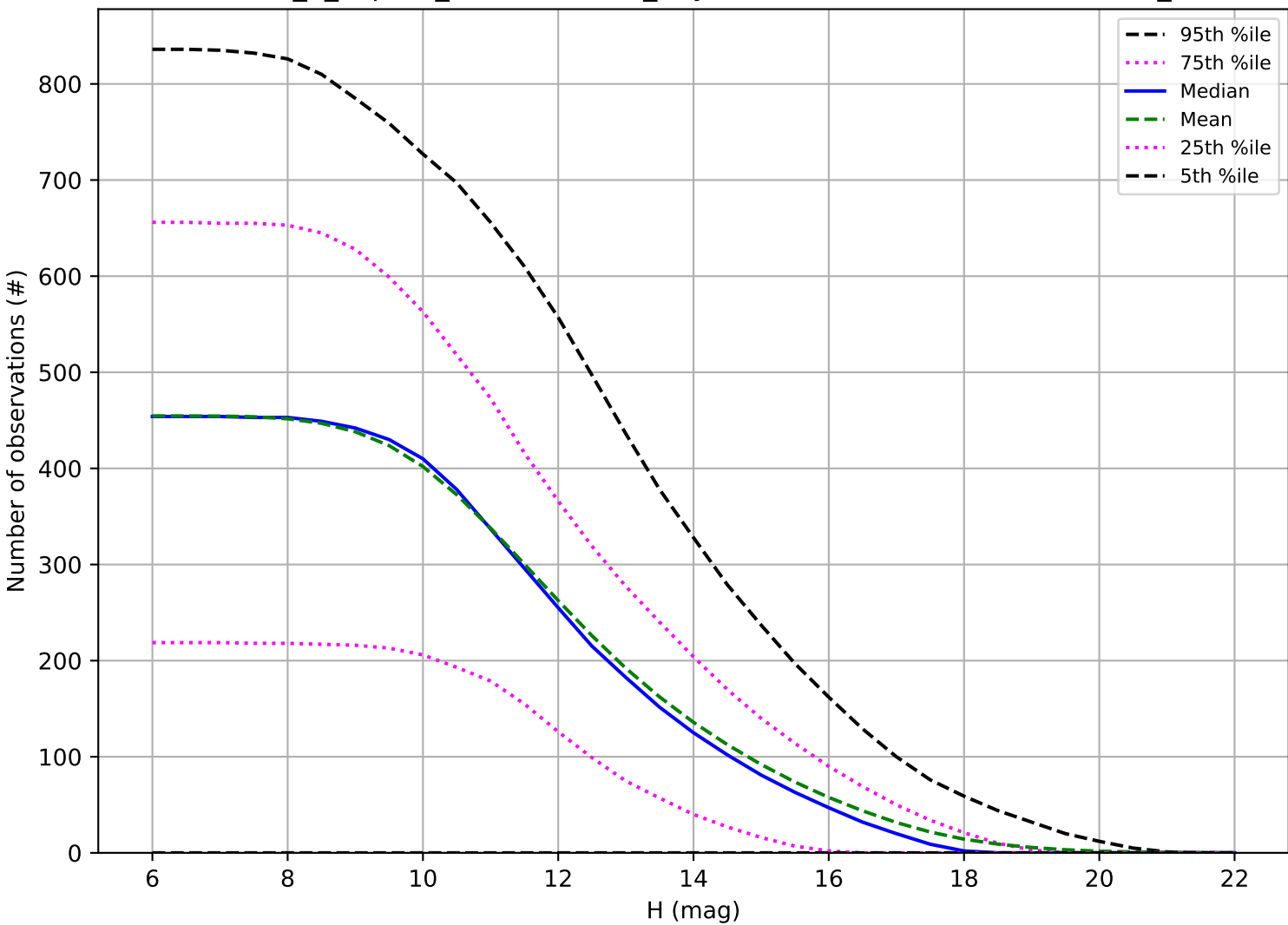
internal_u_expt45_nscale0.9v3.4_10yrs: Number of observations OCC_r5
