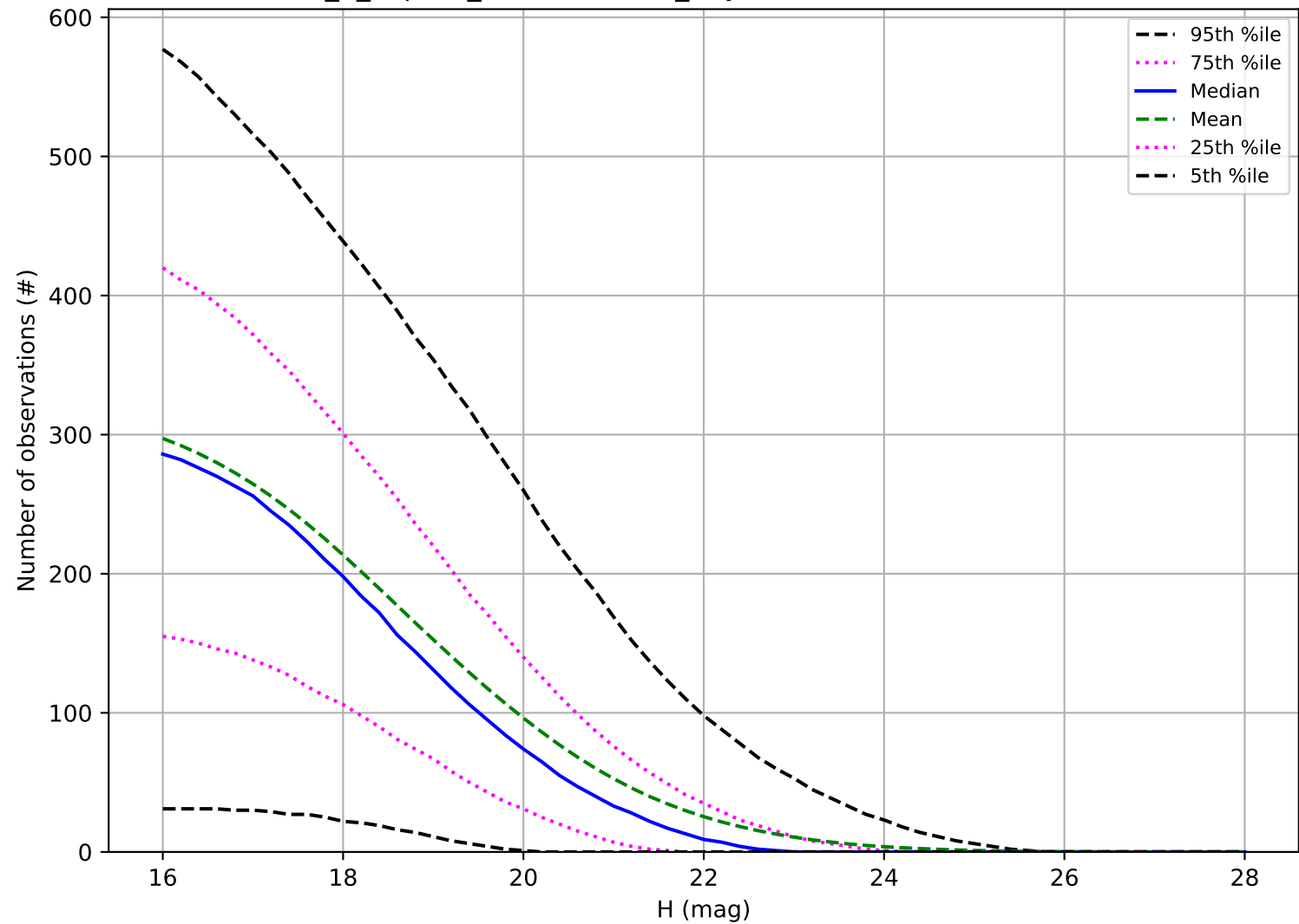
internal_u_expt45_nscale0.9v3.4_10yrs: Number of observations NEO
