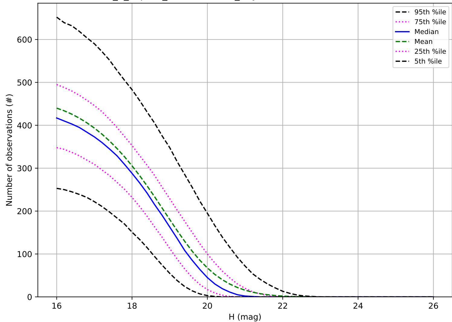
internal_u_expt45_nscale0.9v3.4_10yrs: Number of observations MBA
