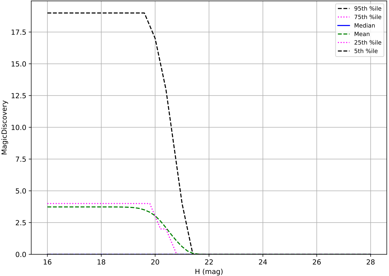
internal_u_expt45_nscale0.9v3.4_10yrs: Vatira 6 detections in 60 nights detection loss
