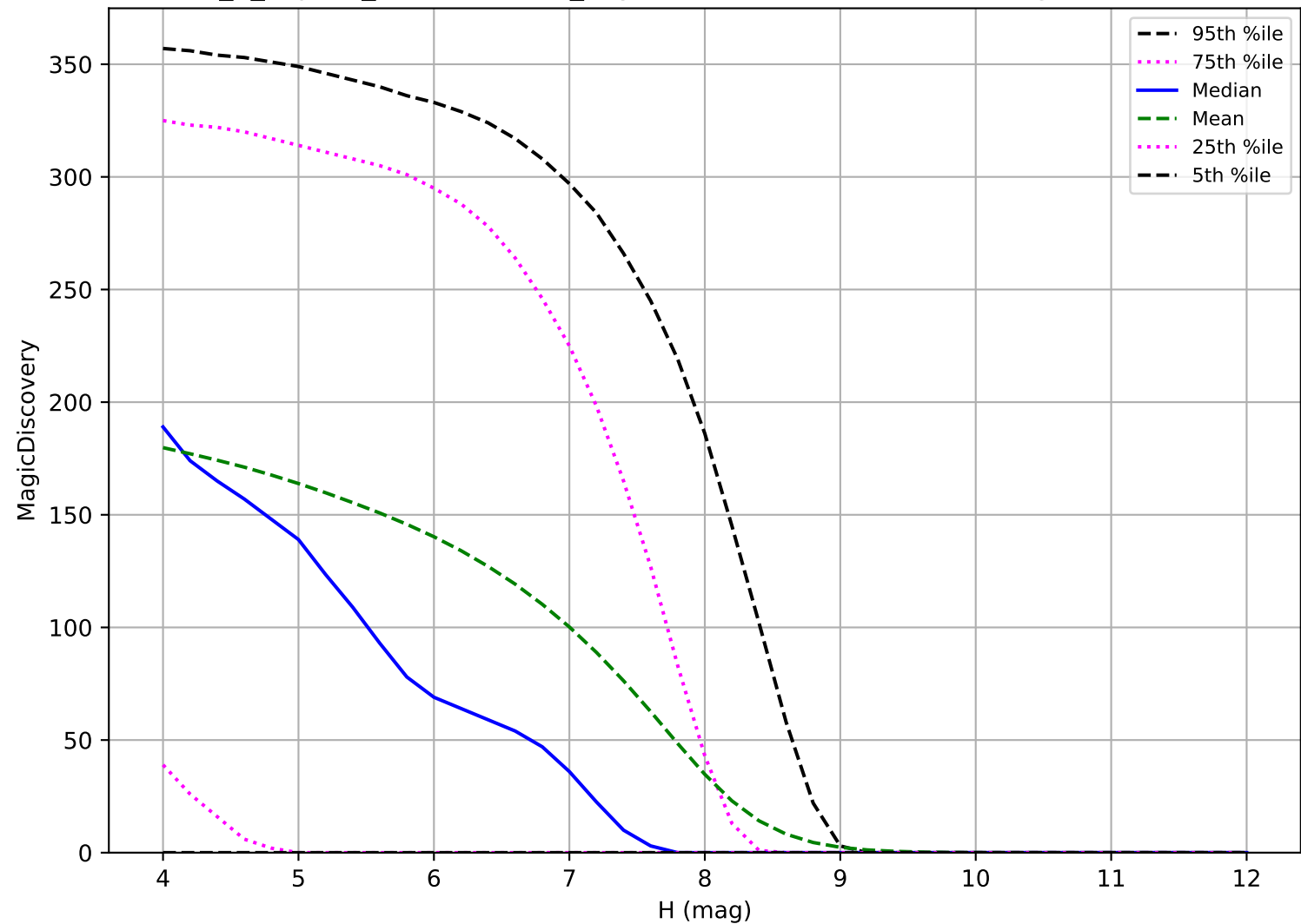
internal_u_expt45_nscale0.9v3.4_10yrs: TNO 6 detections in 60 nights detection loss
