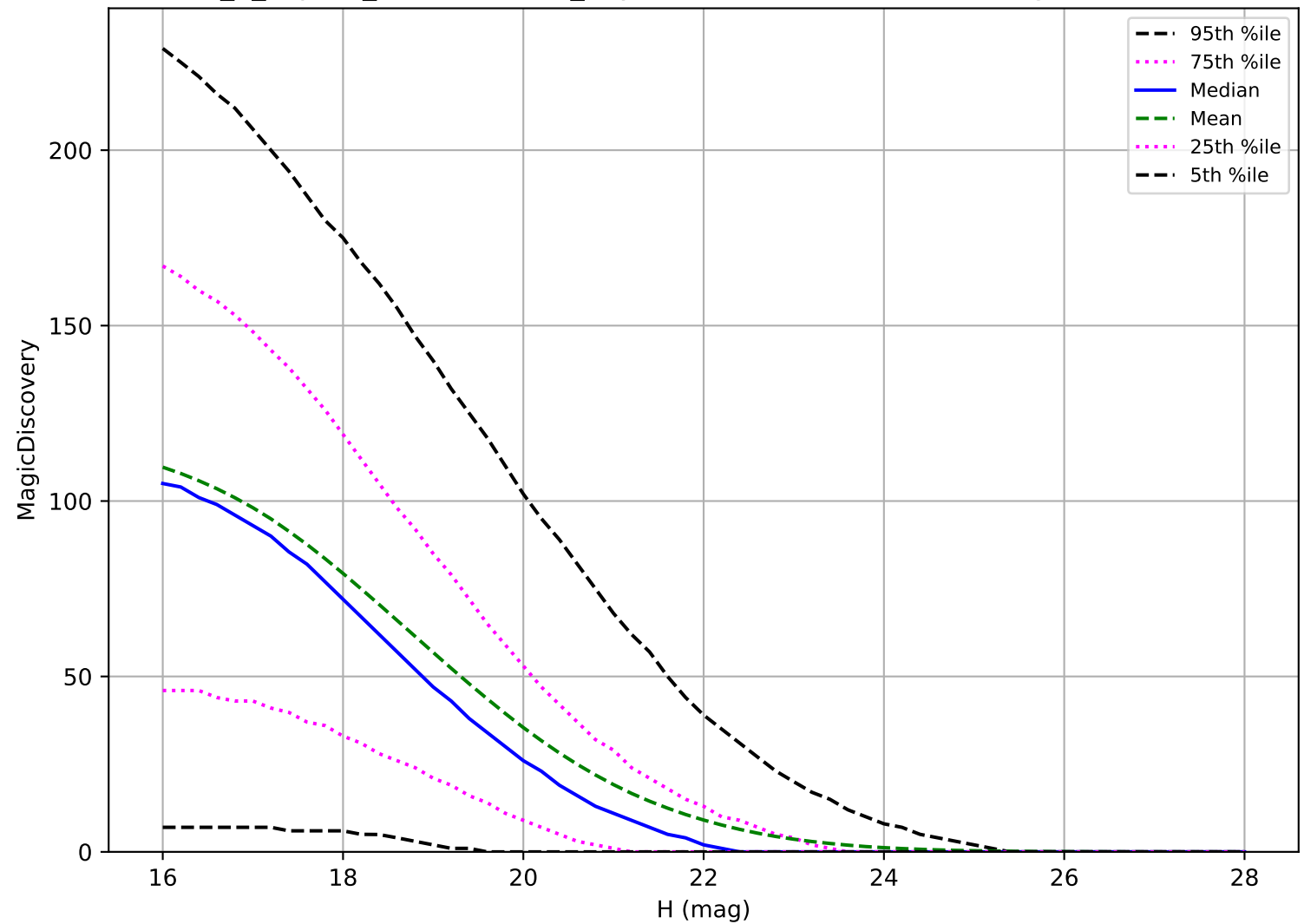
internal_u_expt45_nscale0.9v3.4_10yrs: PHA 6 detections in 60 nights detection loss
