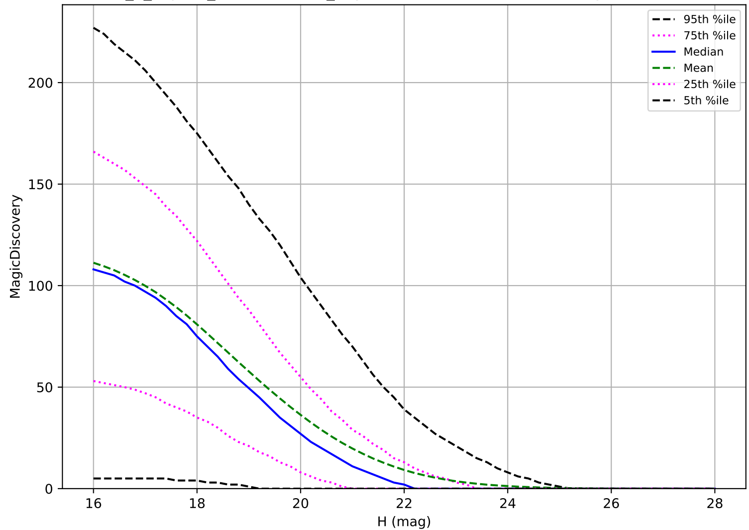
internal_u_expt45_nscale0.9v3.4_10yrs: NEO 6 detections in 60 nights detection loss
