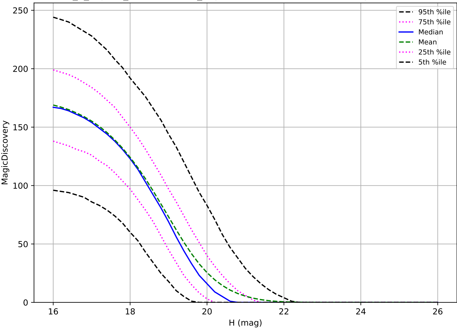
internal_u_expt45_nscale0.9v3.4_10yrs: MBA 6 detections in 60 nights detection loss
