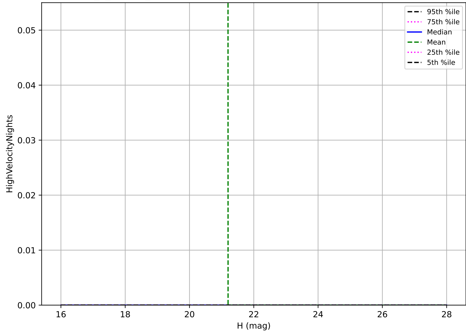
internal_u_expt45_nscale0.9v3.4_10yrs: Vatira High velocity pair detection loss
