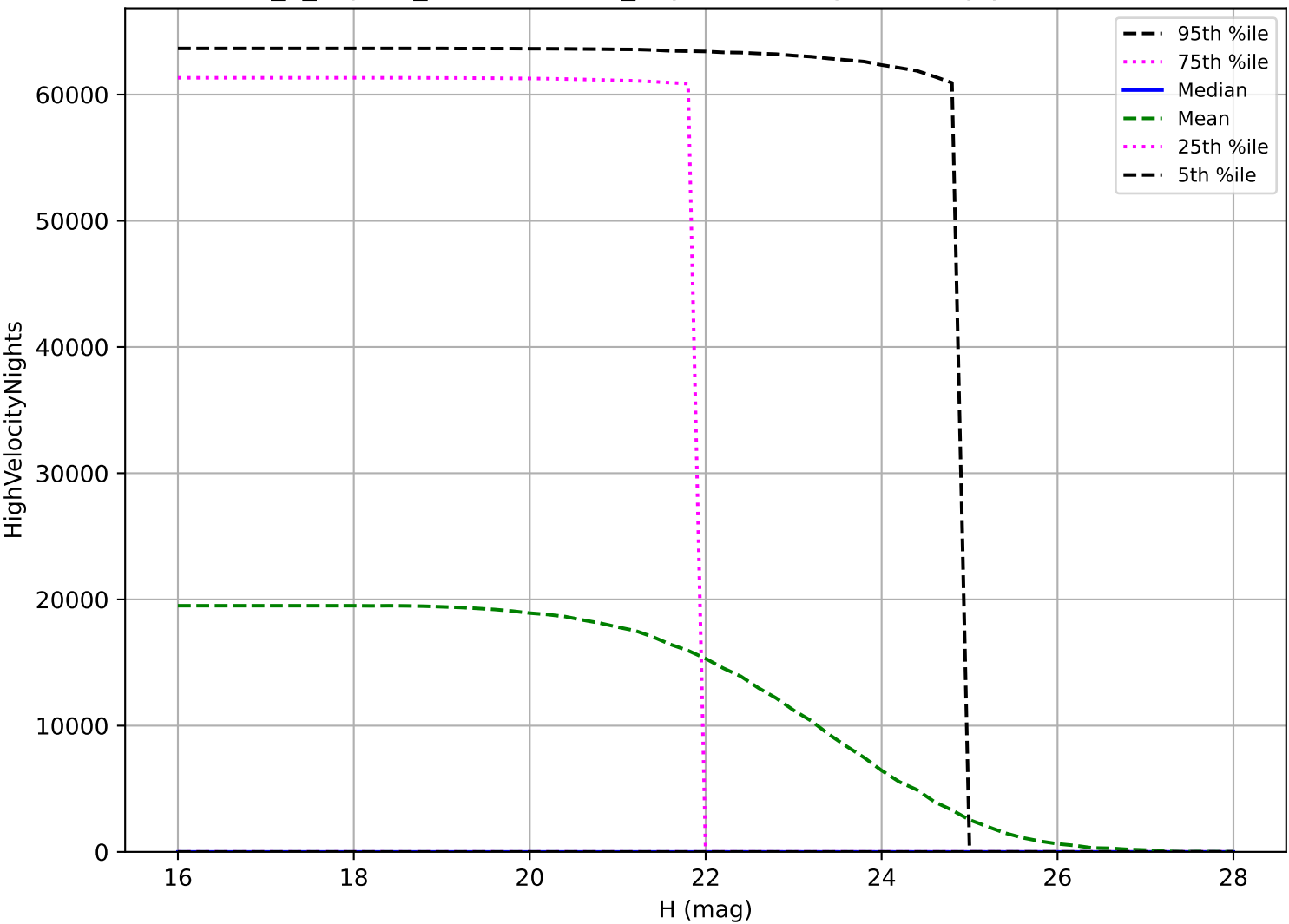
internal_u_expt45_nscale0.9v3.4_10yrs: NEO High velocity pair detection loss
