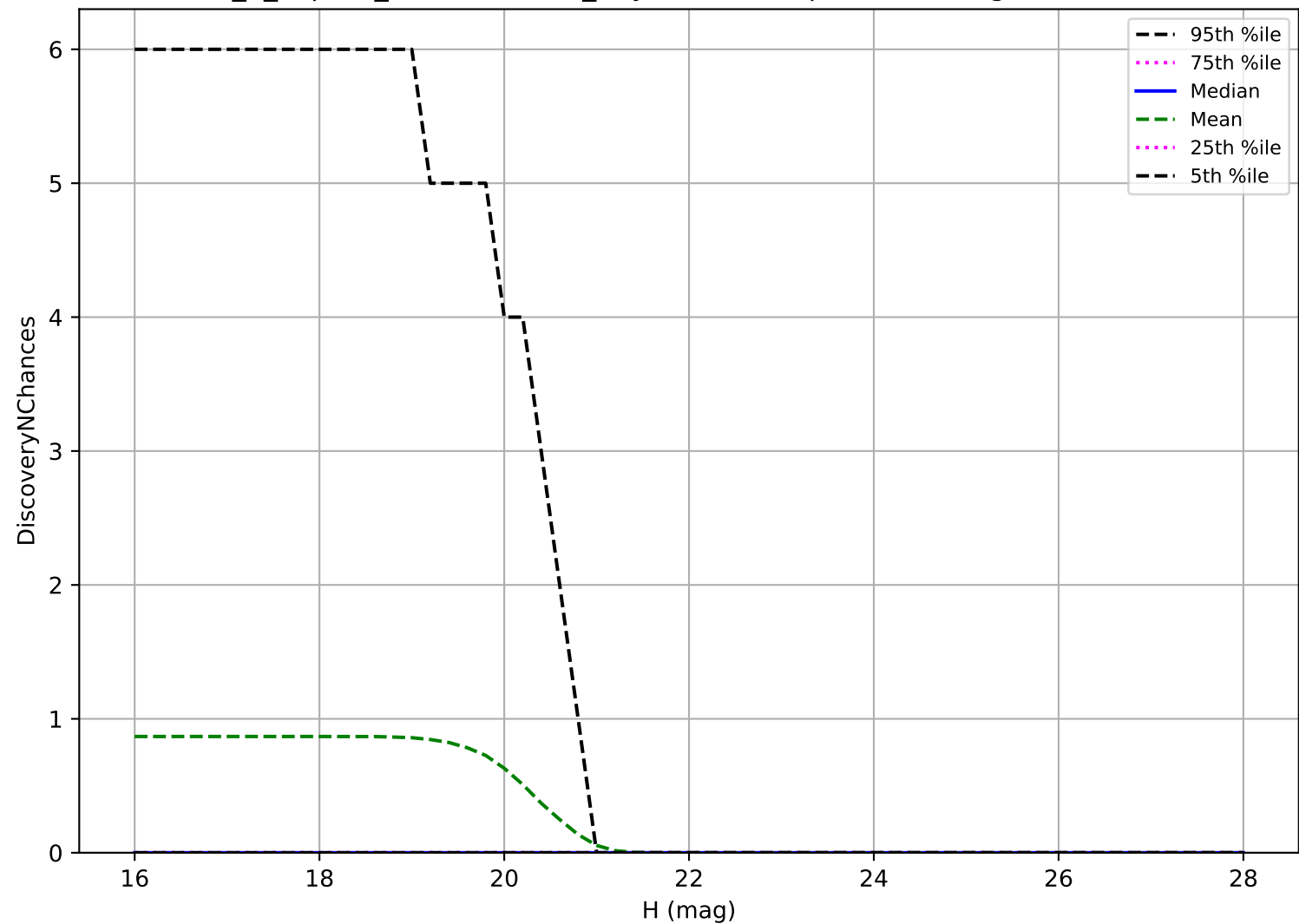
internal_u_expt45_nscale0.9v3.4_10yrs: Vatira 3 pairs in 15 nights detection loss
