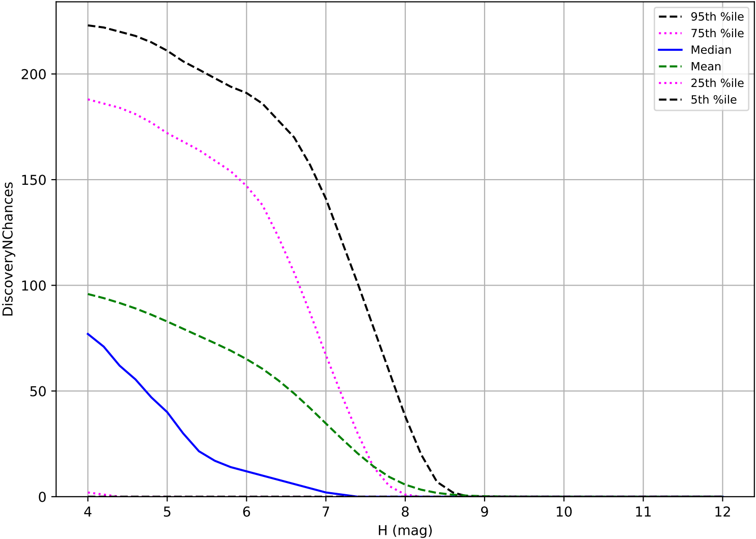
internal_u_expt45_nscale0.9v3.4_10yrs: TNO 3 pairs in 15 nights detection loss
