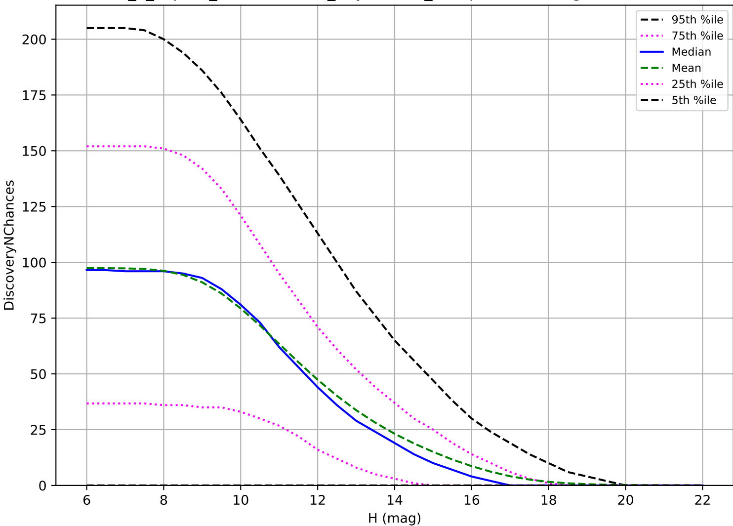
internal_u_expt45_nscale0.9v3.4_10yrs: OCC_r5 3 pairs in 15 nights detection loss
