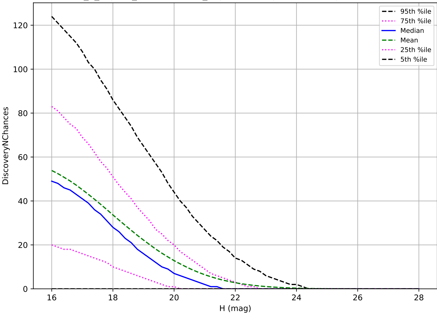
internal_u_expt45_nscale0.9v3.4_10yrs: NEO 3 pairs in 15 nights detection loss
