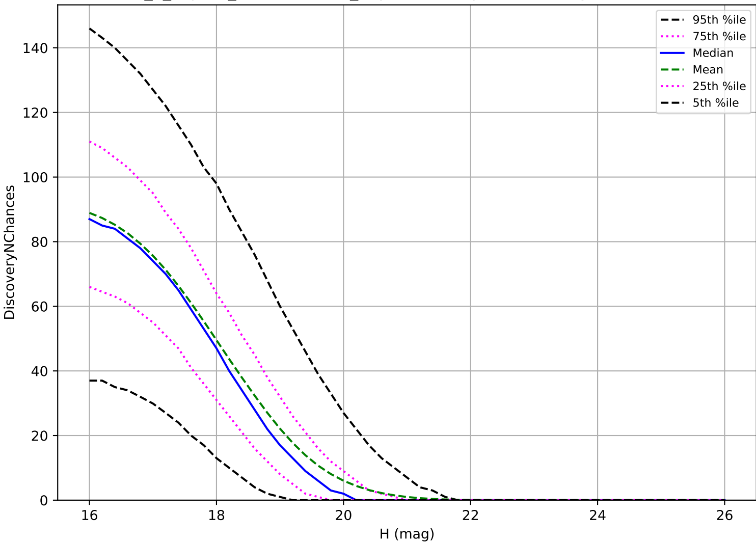
internal_u_expt45_nscale0.9v3.4_10yrs: MBA 3 pairs in 15 nights detection loss
