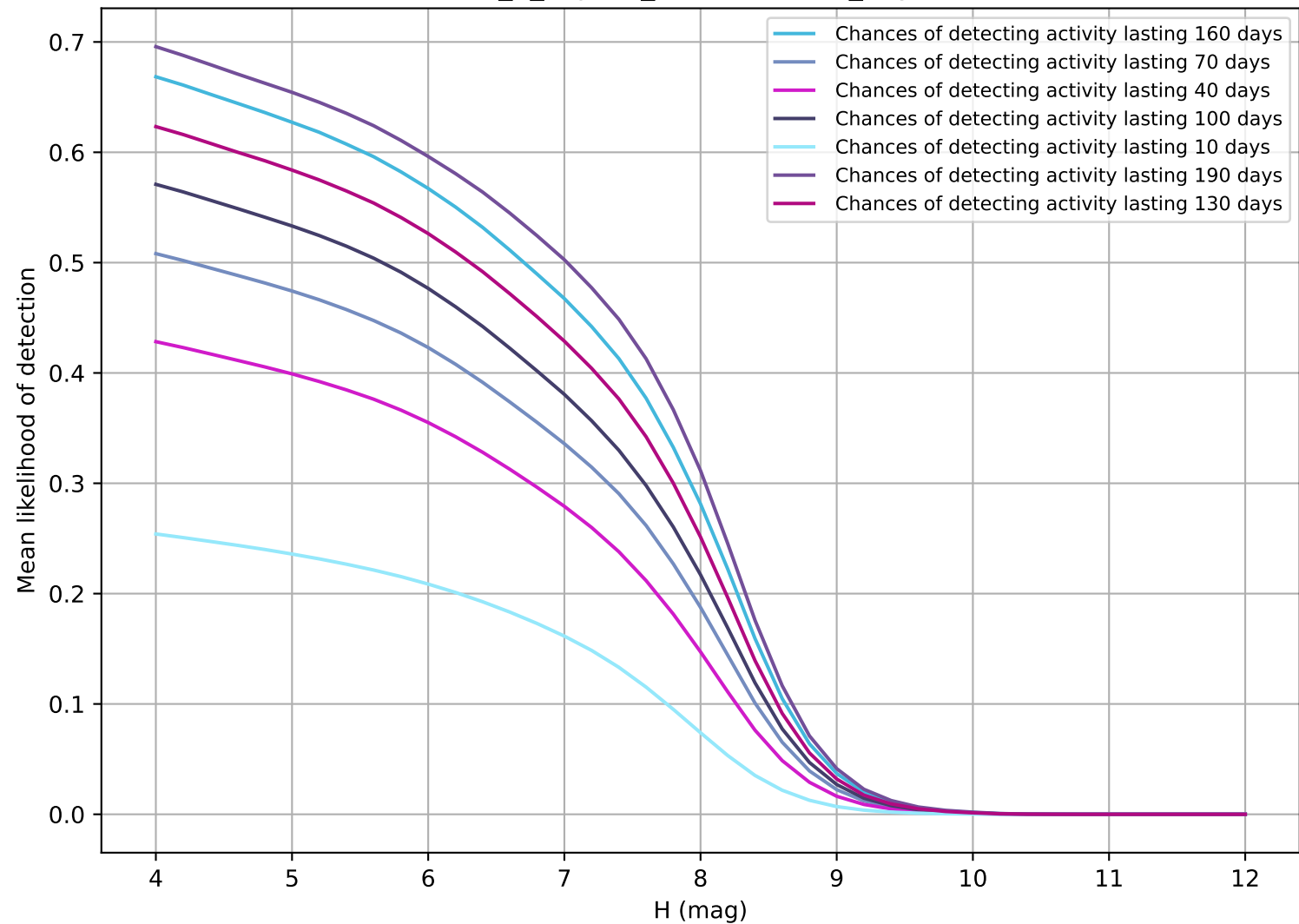
internal_u_expt45_nscale0.9v3.4_10yrs TNO
