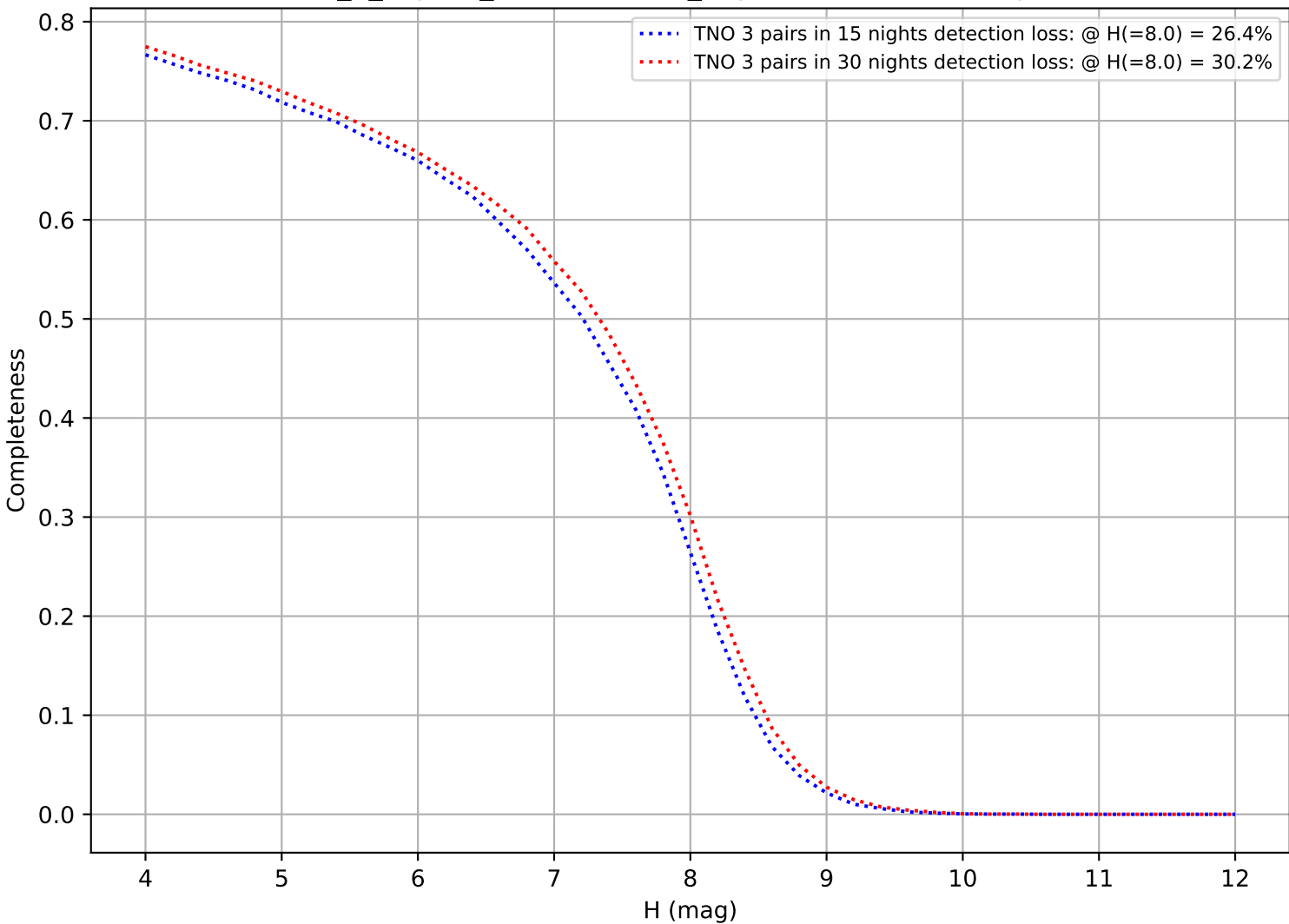
internal_u_expt45_nscale0.9v3.4_10yrs: DifferentialCompleteness
