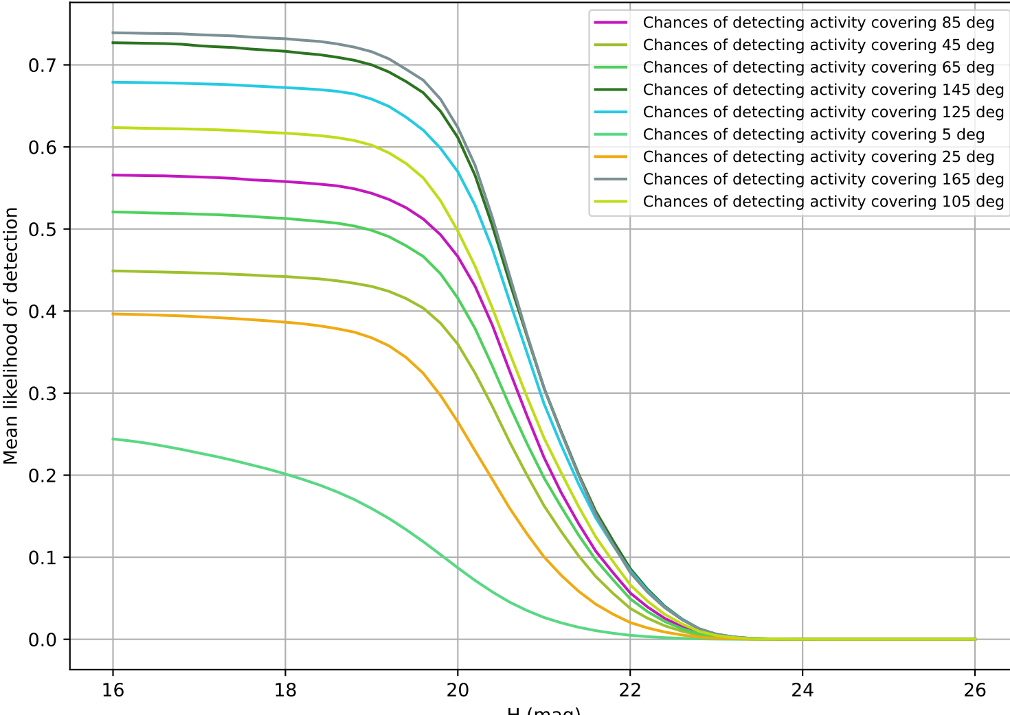
internal u expt45 nscale0.9v3.4 10yrs MBA
