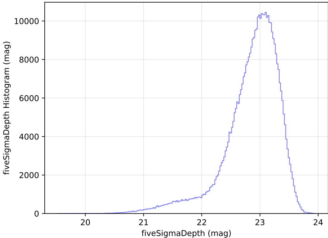
internal_u_expt45_nscale0.9v3.4_10yrs z: fiveSigmaDepth Histogram
