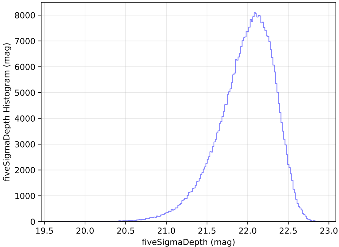
internal_u_expt45_nscale0.9v3.4_10yrs y: fiveSigmaDepth Histogram
