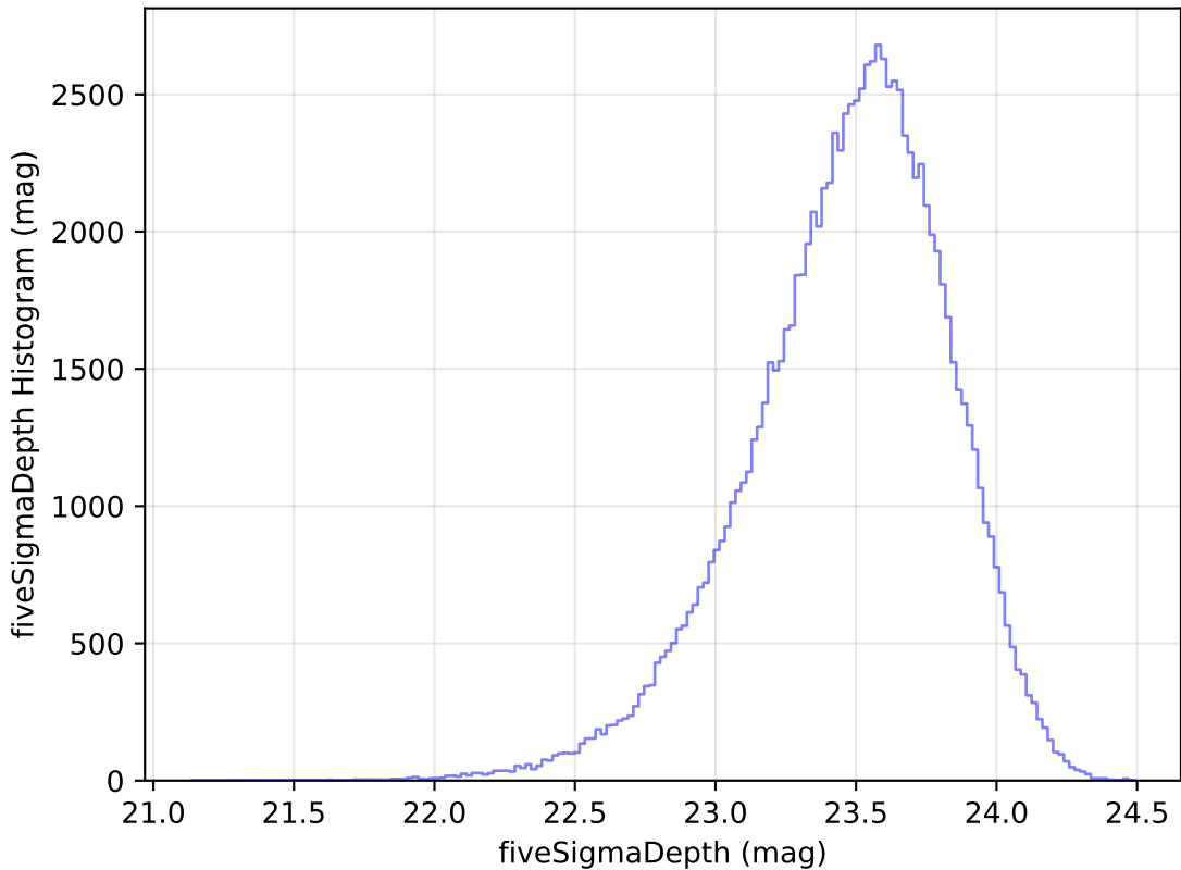
internal_u_expt45_nscale0.9v3.4_10yrs u: fiveSigmaDepth Histogram
