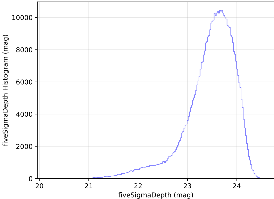
internal_u_expt45_nscale0.9v3.4_10yrs i: fiveSigmaDepth Histogram
