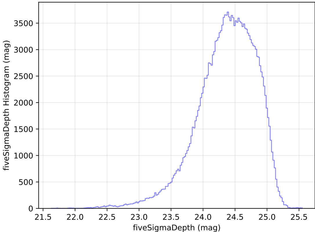
internal_u_expt45_nscale0.9v3.4_10yrs g: fiveSigmaDepth Histogram
