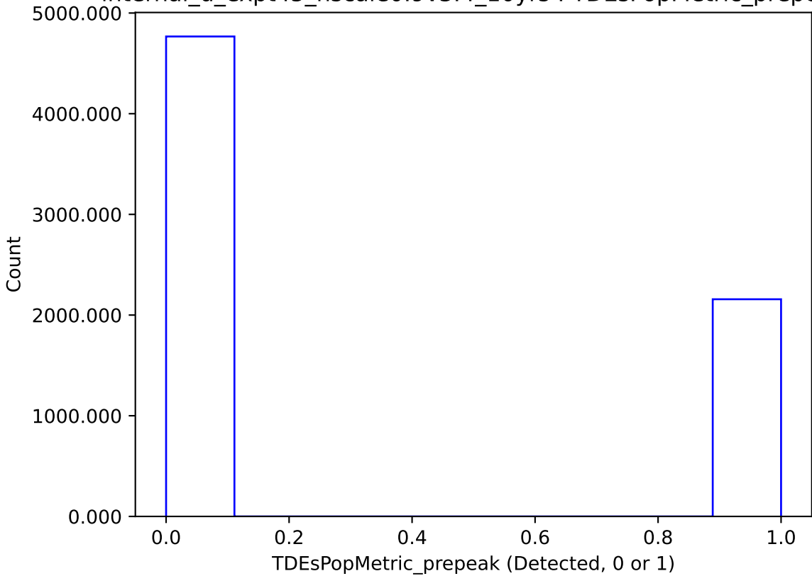
internal_u_expt45_nscale0.9v3.4_10yrs : TDEsPopMetric_prepeak
