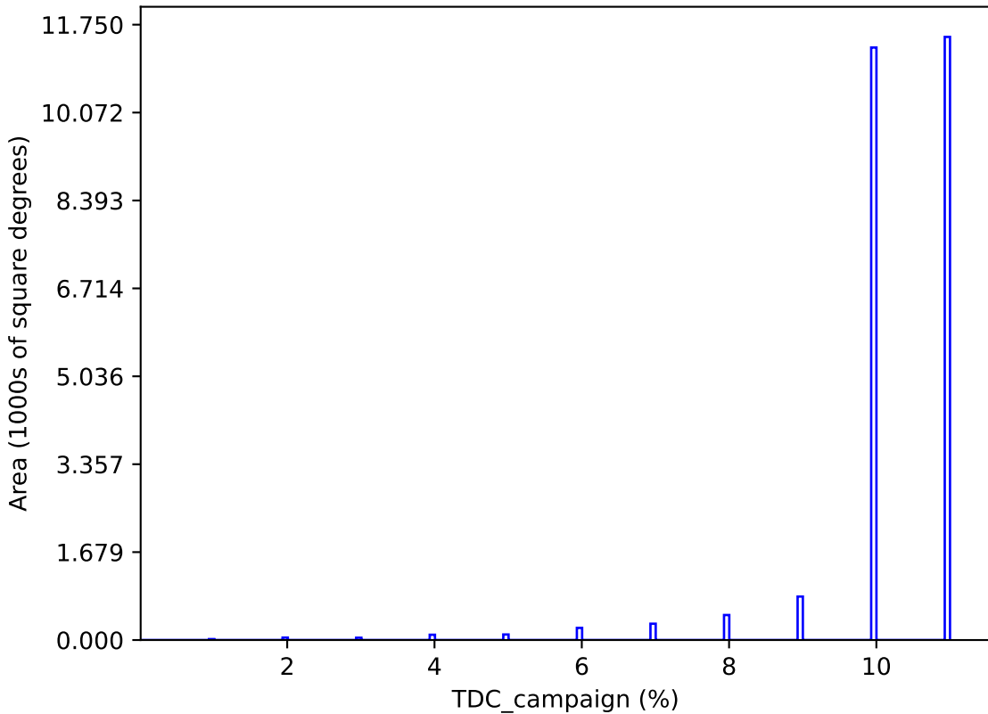
internal_u_expt45_nscale0.9v3.4_10yrs : TDC_campaign
