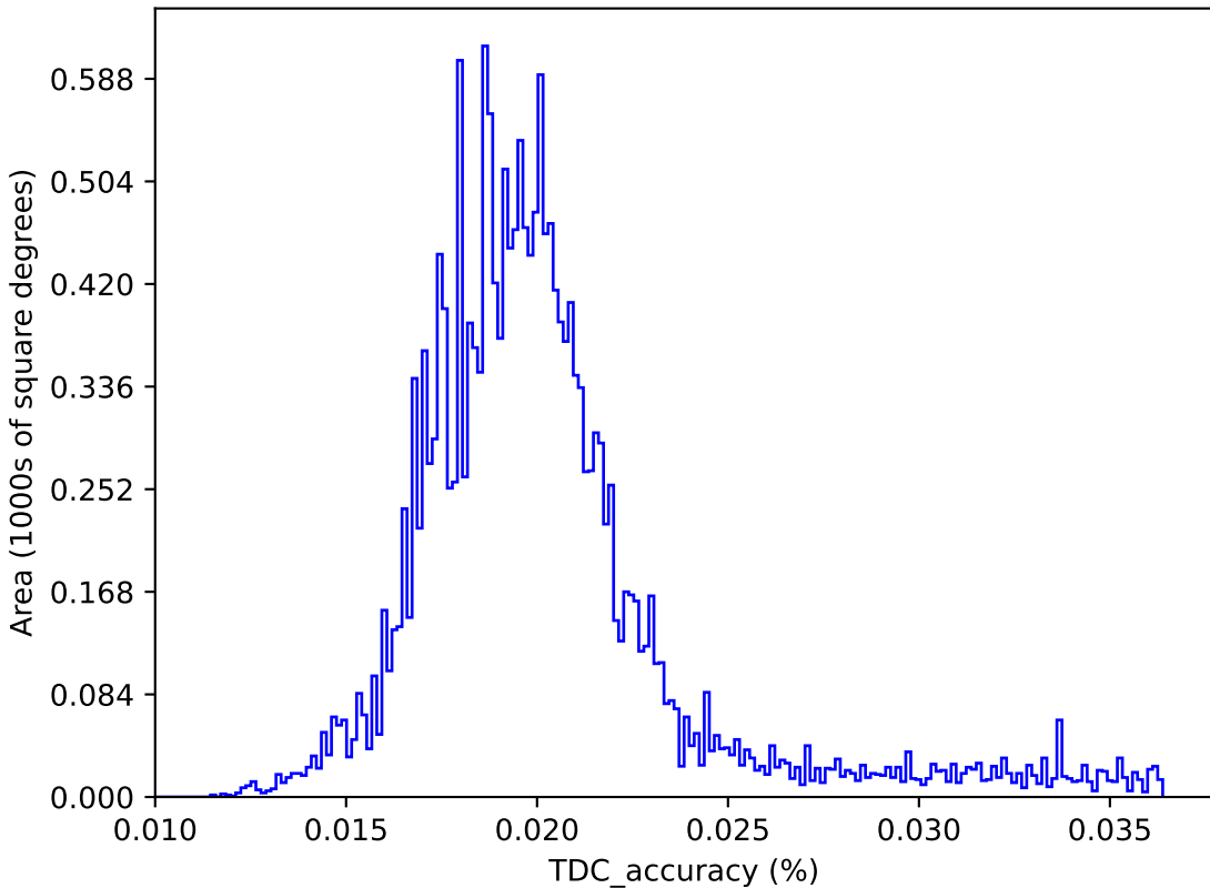
internal_u_expt45_nscale0.9v3.4_10yrs : TDC_accuracy
