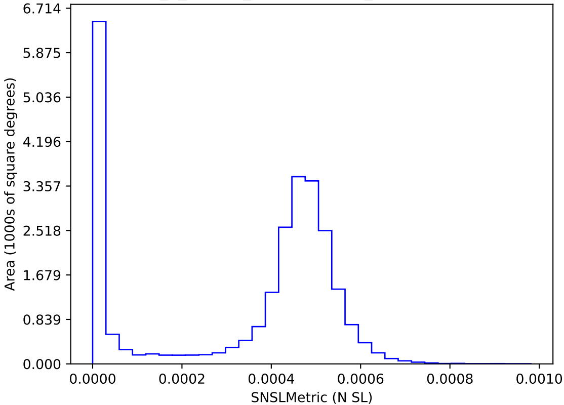
internal_u_expt45_nscale0.9v3.4_10yrs : SNSLMetric
