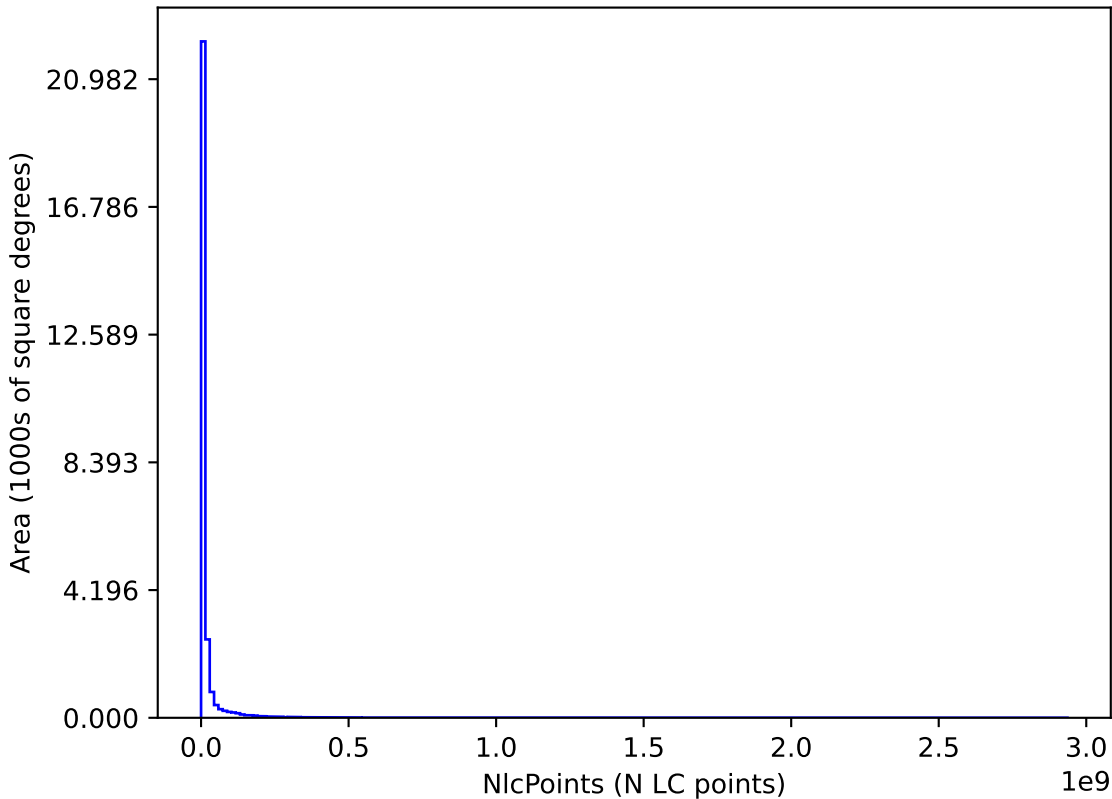
internal_u_expt45_nscale0.9v3.4_10yrs : NlcPoints
