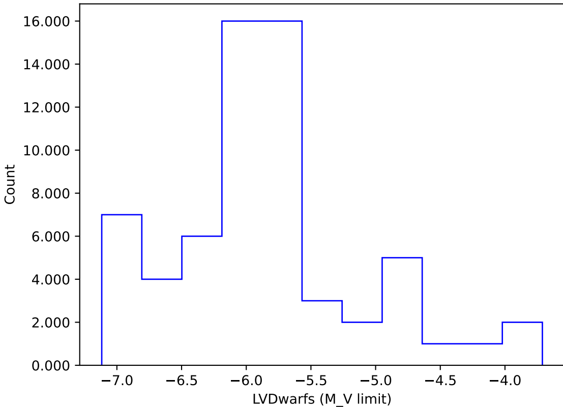
internal_u_expt45_nscale0.9v3.4_10yrs gi: LVDwarfs
