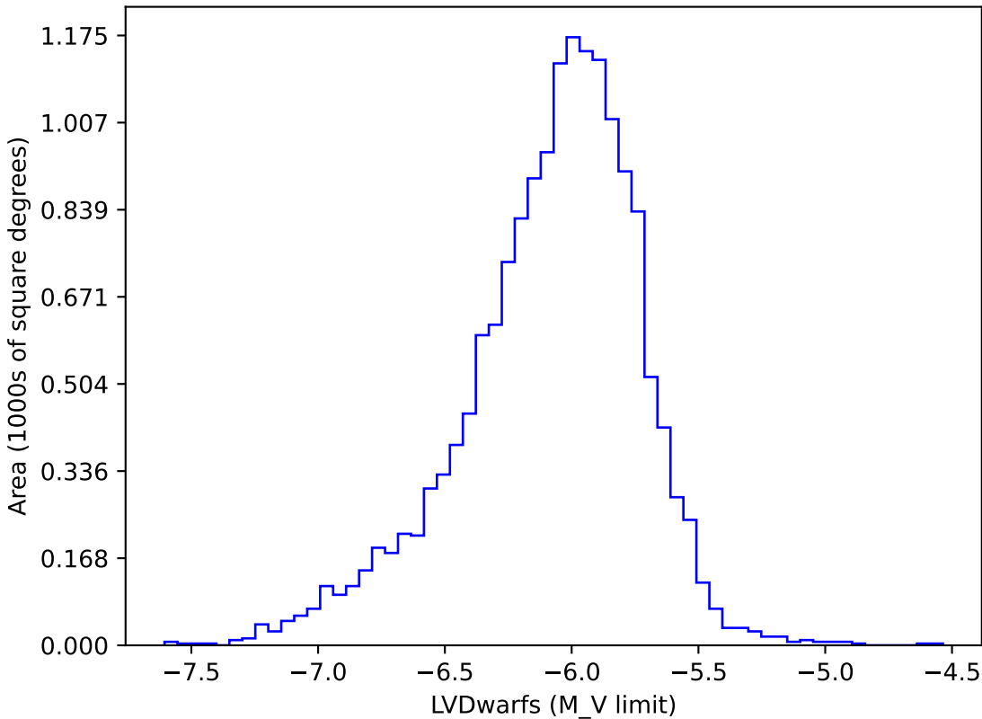
internal_u_expt45_nscale0.9v3.4_10yrs gi: LVDwarfs
