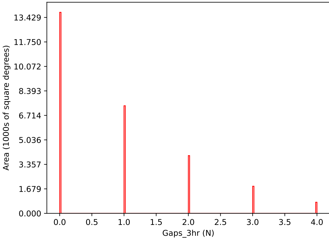
internal_u_expt45_nscale0.9v3.4_10yrs i band: Gaps_3hr
