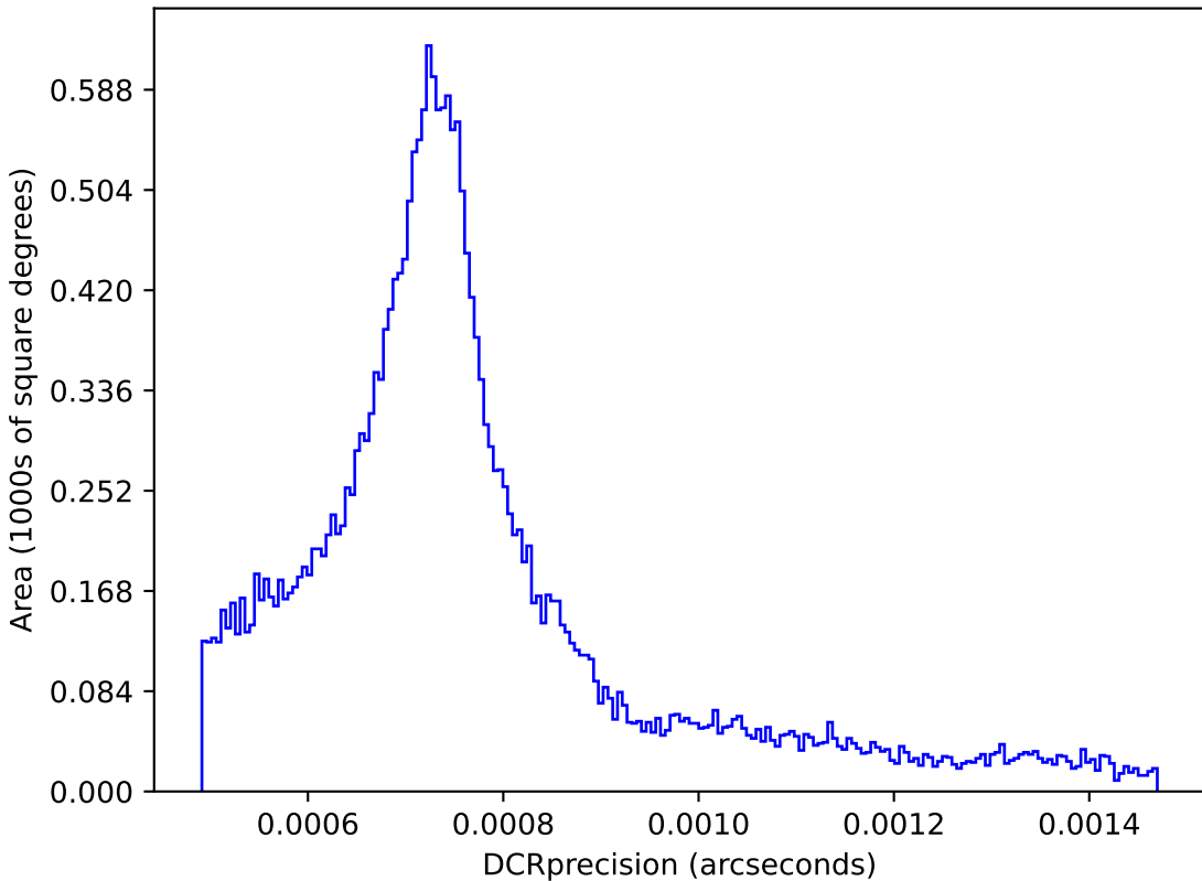
internal_u_expt45_nscale0.9v3.4_10yrs : DCRprecision
