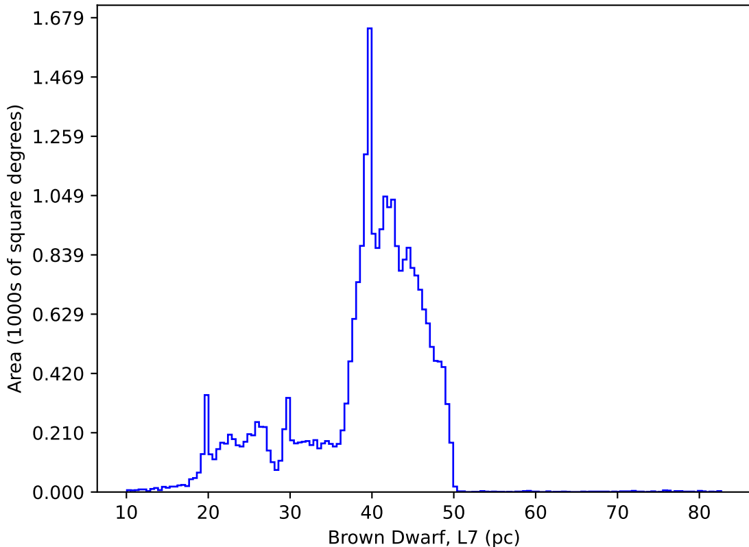
internal_u_expt45_nscale0.9v3.4_10yrs : Brown Dwarf, L7
