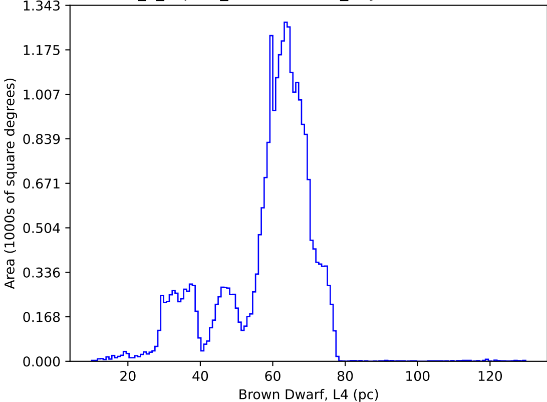
internal_u_expt45_nscale0.9v3.4_10yrs : Brown Dwarf, L4
