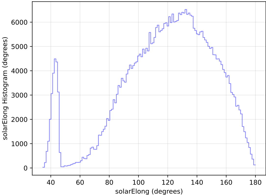
internal_u_expt45_nscale0.9v3.4_10yrs WFD z band: solarElong Histogram
