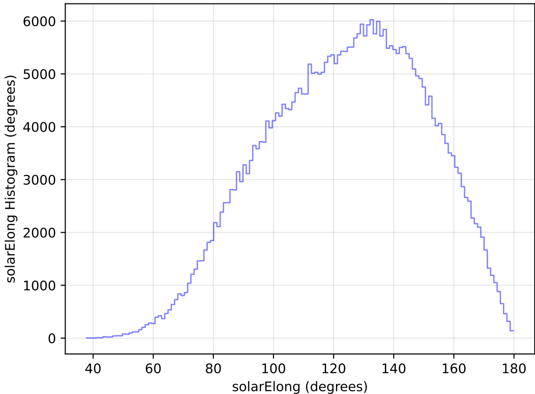
internal_u_expt45_nscale0.9v3.4_10yrs WFD y band: solarElong Histogram
