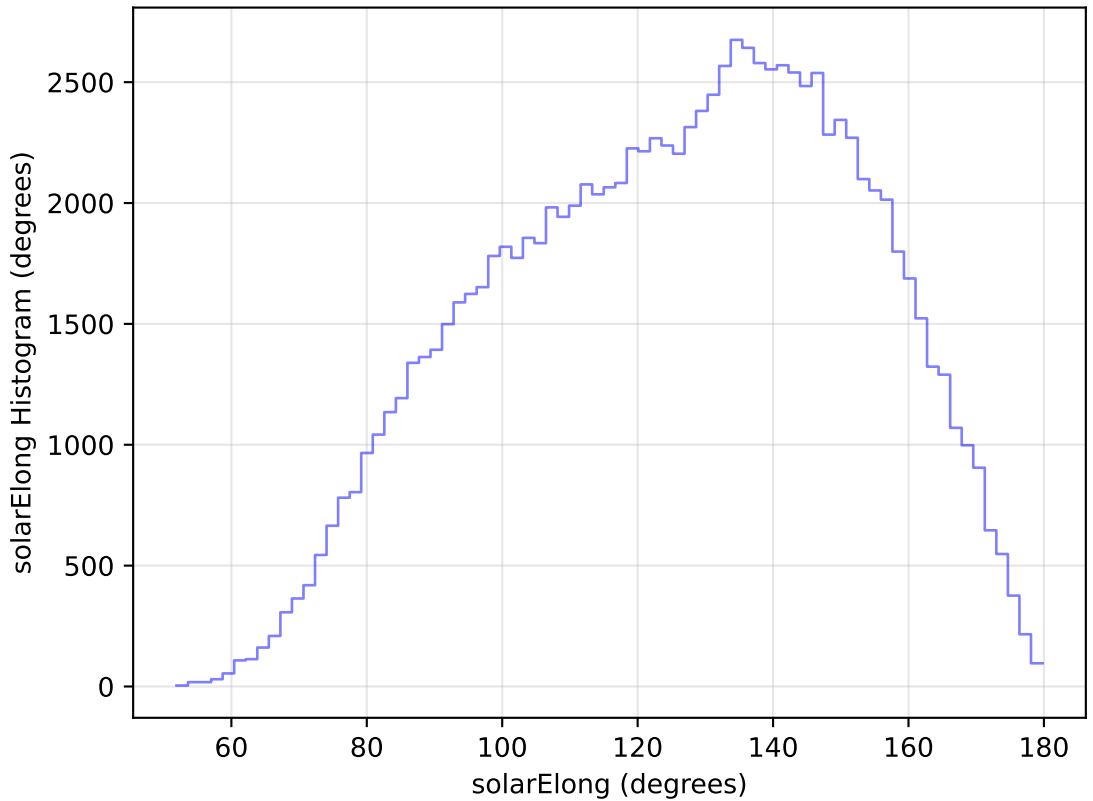
internal_u_expt45_nscale0.9v3.4_10yrs WFD u band: solarElong Histogram
