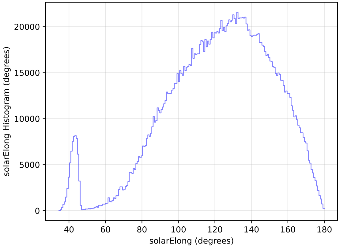
internal_u_expt45_nscale0.9v3.4_10yrs WFD all bands: solarElong Histogram
