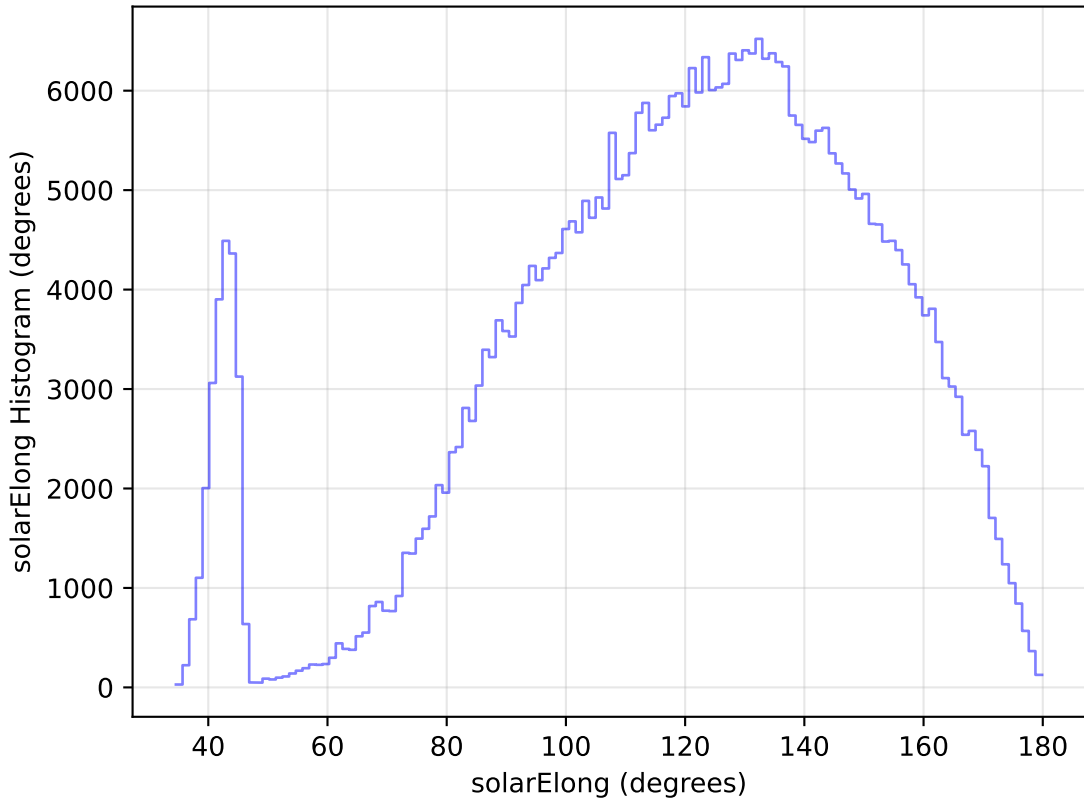
internal_u_expt45_nscale0.9v3.4_10yrs All sky z band: solarElong Histogram
