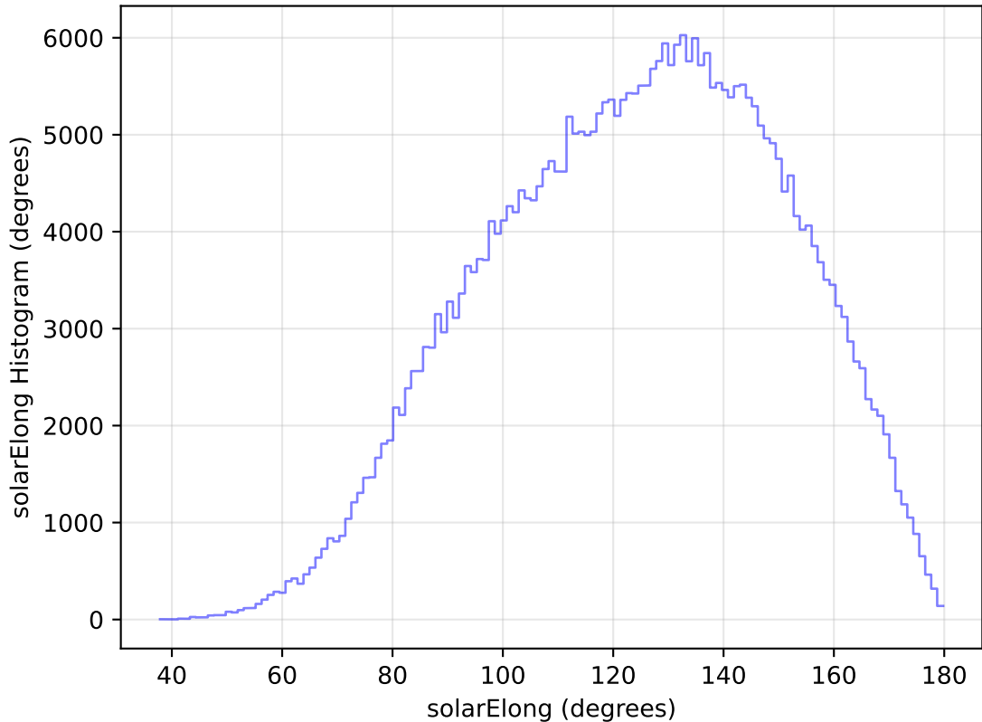
internal_u_expt45_nscale0.9v3.4_10yrs All sky y band: solarElong Histogram
