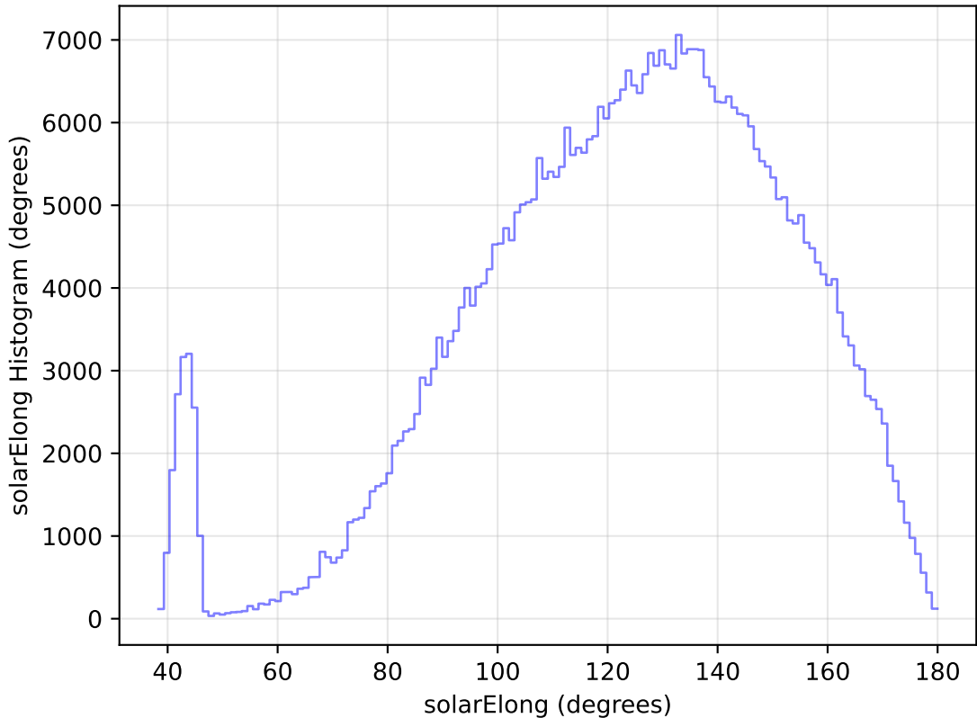
internal_u_expt45_nscale0.9v3.4_10yrs All sky r band: solarElong Histogram
