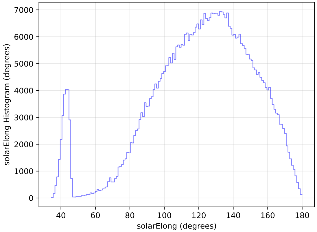
internal_u_expt45_nscale0.9v3.4_10yrs All sky i band: solarElong Histogram
