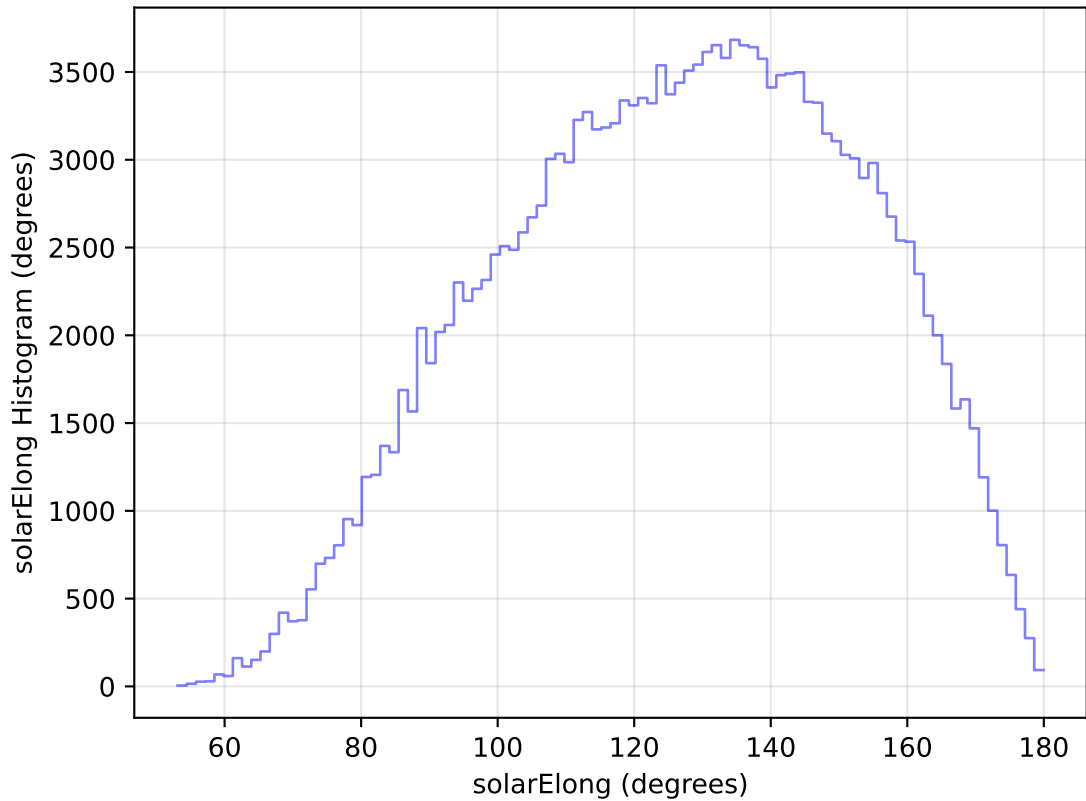
internal_u_expt45_nscale0.9v3.4_10yrs All sky g band: solarElong Histogram
