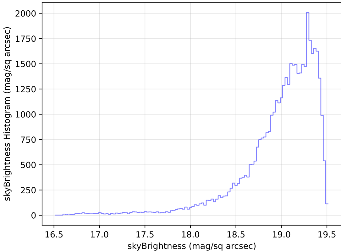
internal_u_expt45_nscale0.9v3.4_10yrs Yr 1 z band: skyBrightness Histogram
