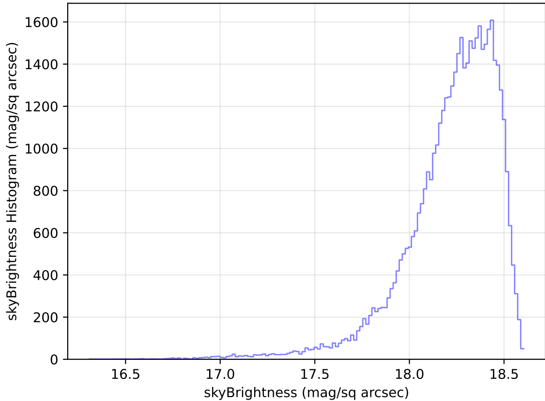
internal_u_expt45_nscale0.9v3.4_10yrs Yr 1 y band: skyBrightness Histogram
