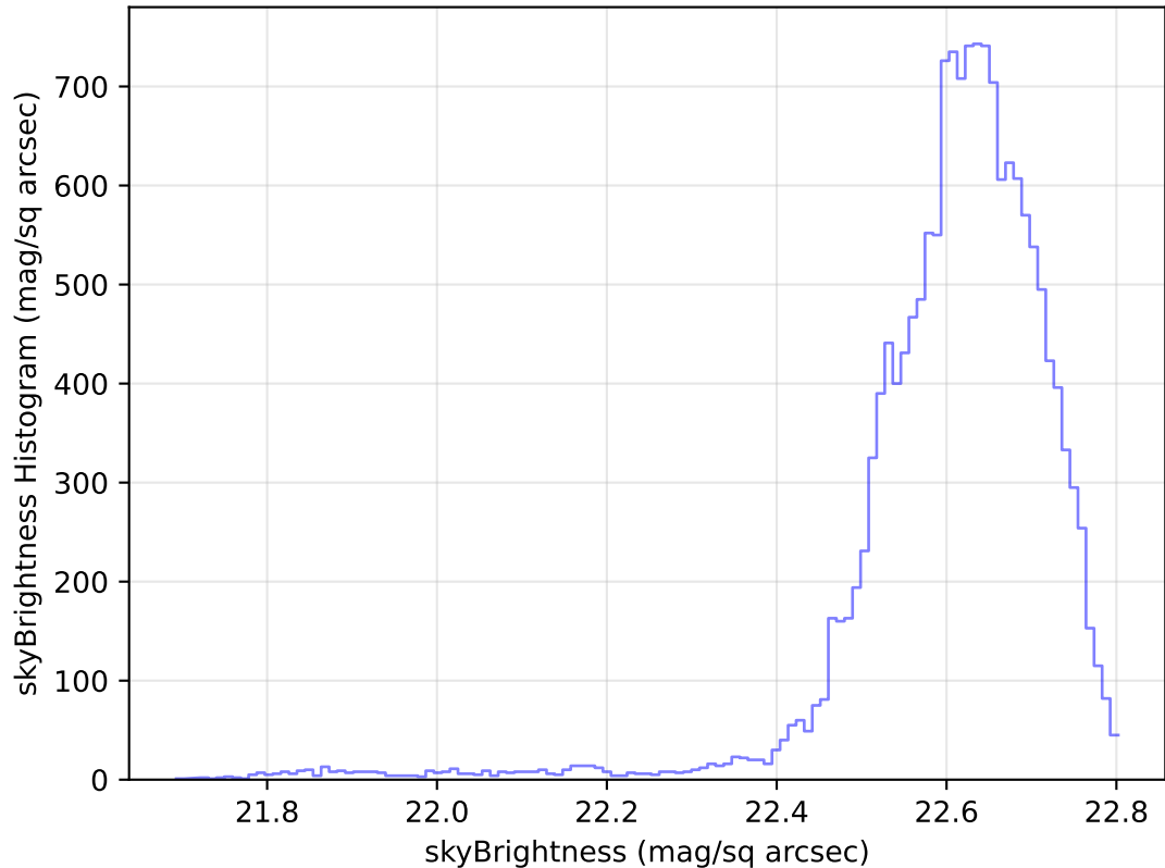
internal_u_expt45_nscale0.9v3.4_10yrs Yr 1 u band: skyBrightness Histogram
